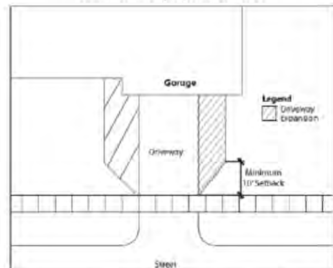
Figure 10-104c Minimum Driveway Expansion Setback
